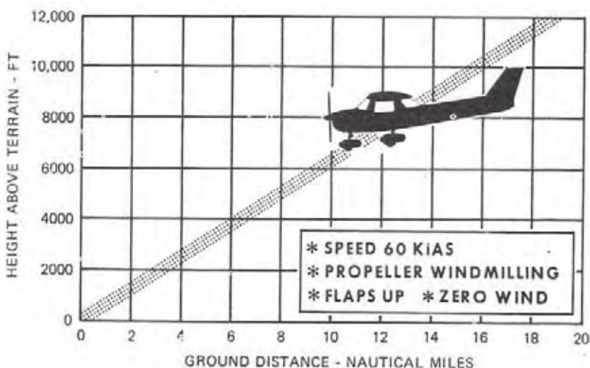
Figure 3-1. Maximum Glide
