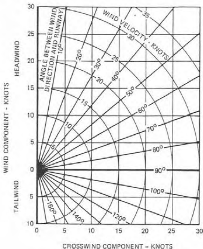
Figure 5-4. Wind Components
