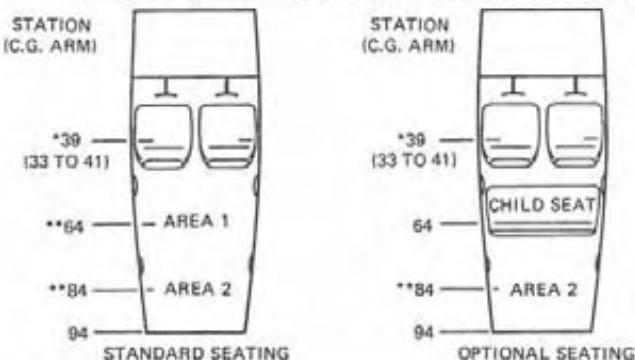
Figure 6-3. Loading Arrangements
