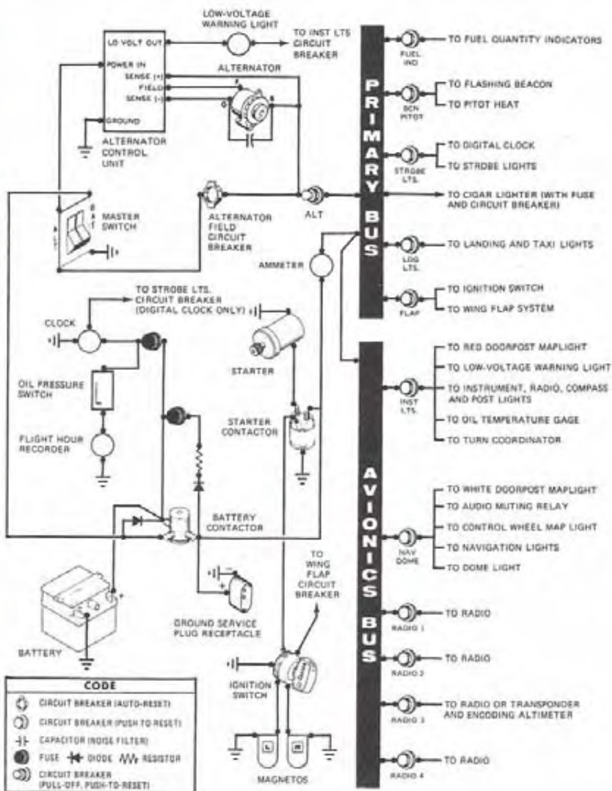
Figure 7-7. Electrical System
